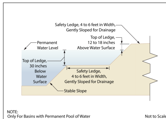
Figure 1. Elevation View - Basin Safety Ledge Configuration
